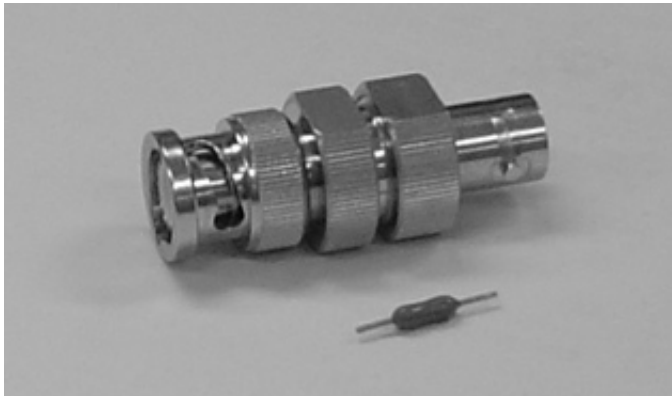
BNC Fuse Adapter and 0.125 A Fuse
