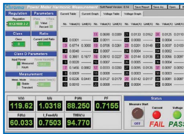
IEC 61000-3-2 Current Harmonic Test
