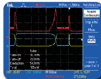
► Figure 9: TPS Series' switching loss display showing turn-on, turn-off and conduction losses
