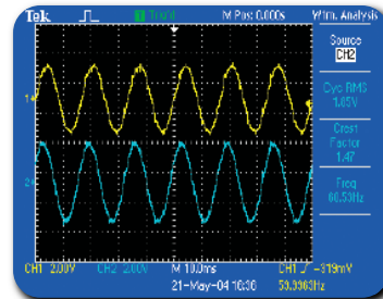
► Figure 7: TPS Series' waveform analysis
