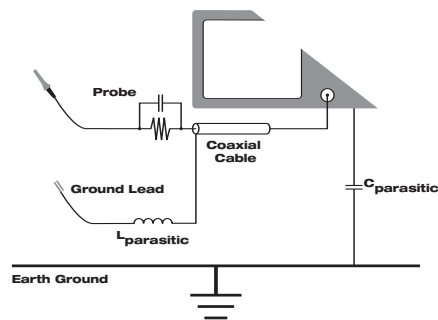
► Figure A: Parasitic inductance and capacitance can affect measurement quality.
