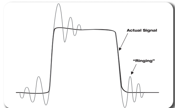
► Figure 2: Ringing caused by parasitic inductance and capacitance distorts the signal and invalidates measurements.
