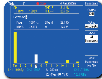
► Figure 5: Harmonic distortion measurements
