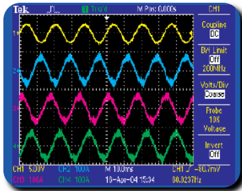
► Figure 4: The 4-channel TPS2024 oscilloscope's channel-to-channel isolation eliminates cross-talk effects when large and small signals are captured simultaneously.
