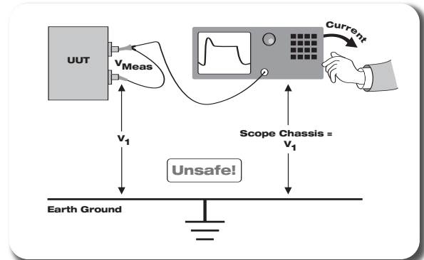
► Figure 1: A floating measurement in which dangerous voltages occur on the oscilloscope chassis. V_1 may be hundreds of volts!
