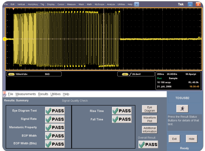
▶ Figure 3. Measurement results are automatically displayed using the TDSUSB2 compliance test package.
