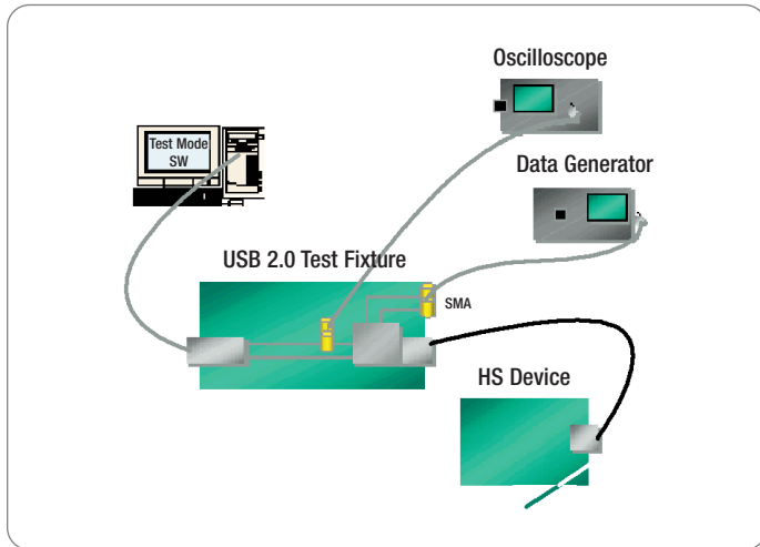
► Figure 5. Set-up for a receiver sensitivity test using a DPO7254 and DTG5000 data generator.
