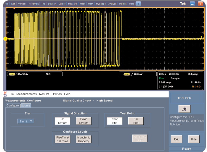
▶ Figure 2. TDSUSB2 compliance test package running on a DP07254.
