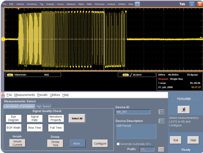
▶ Figure 1. TDSUSB2 compliance test package running on a DP07254.
