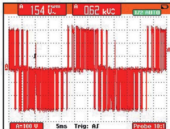
Figure 6: Motor drive output measured using the Fluke 199C
