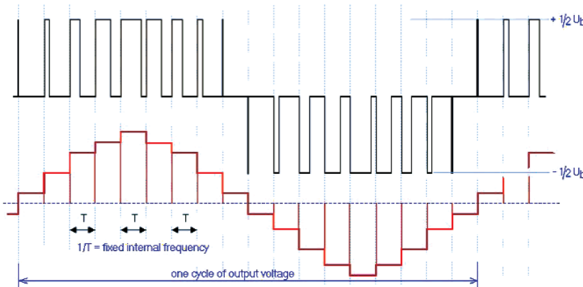
Figure 5: Output voltages for pulse-width-modulated motor drive (simplified).
