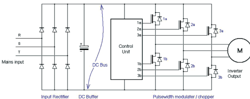
Figure 2: Basic structure of a variable-speed motor drive.
