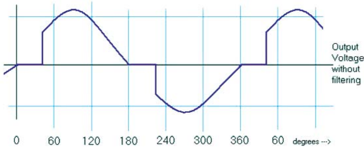
Figure 1: Output voltage of SCR-based power converter. The unfiltered output voltage clearly shows discontinuities.
