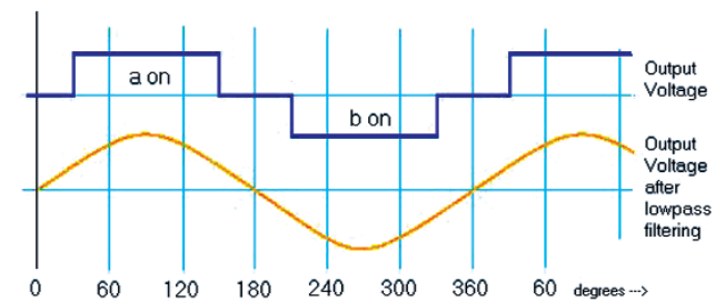
Figure 4: Output voltage directly and through a low-pass filter.
